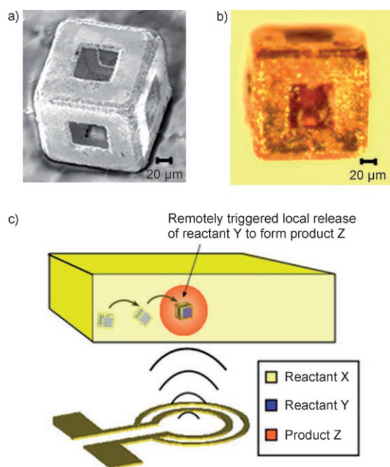
Figure 1. a) A scanning electron microscope image of an empty container. The containers were three-dimensional (3D) porous cubes with a length of approximately 200 µm and a volume of 8 nL. b) An optical microscope image of a container loaded with a dye-soaked pluronic gel. c) A schematic diagram of the experimental set-up used to facilitate wireless microscale chemical engineering (not drawn to scale). Containers were manipulated using a magnetic stylus (not shown) and the contents of specific containers were released by directing an RF source towards the container. In the schematic representation, chemical Y is released from a specific container; chemical Y then reacts with chemical X in the surrounding medium to form product Z.
